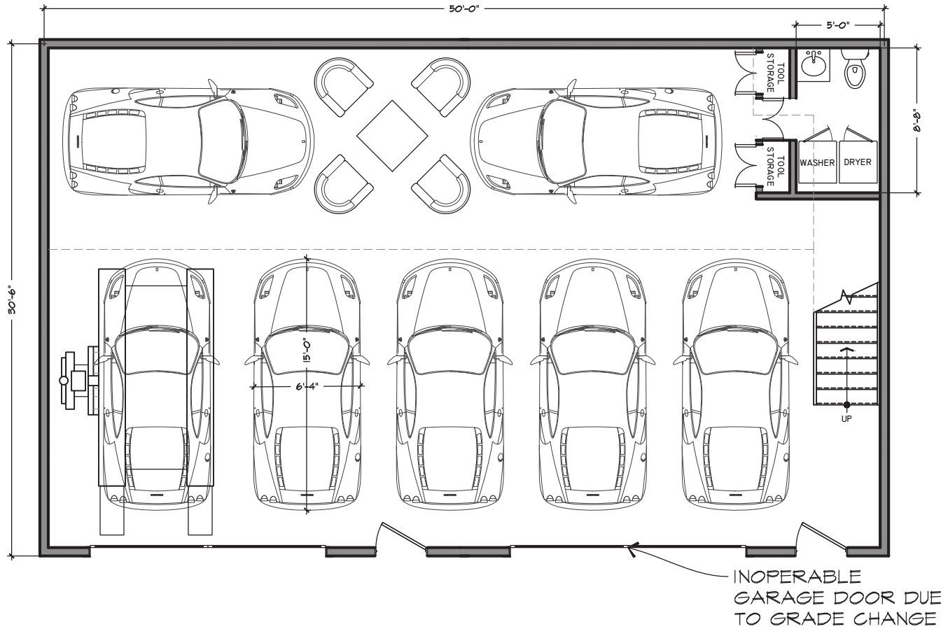
2 UNIT E: OPTION 3 (GROUND FLOOR) SCALE: 1/8" = 1'-0"
